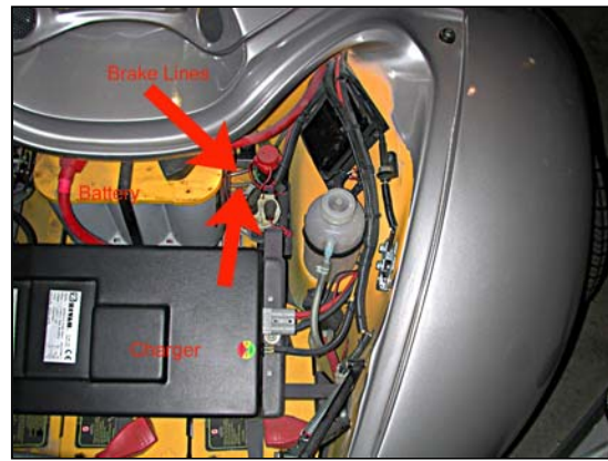
Inadequately secured brake lines on Right Side
